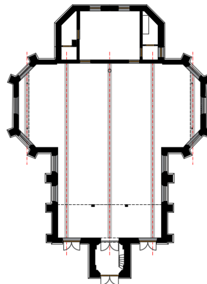
FUNDERINGSPLAN
